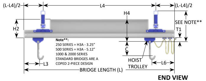
COPED ALUMIINUM TRACK BRIDGE ON STEEL RUNWAYS
